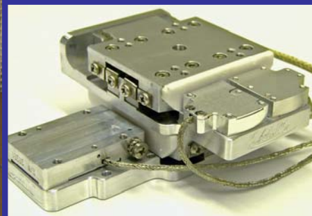
Dual Miniature Goniometer Stack
