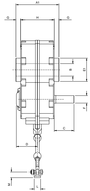
Keyed Hub
